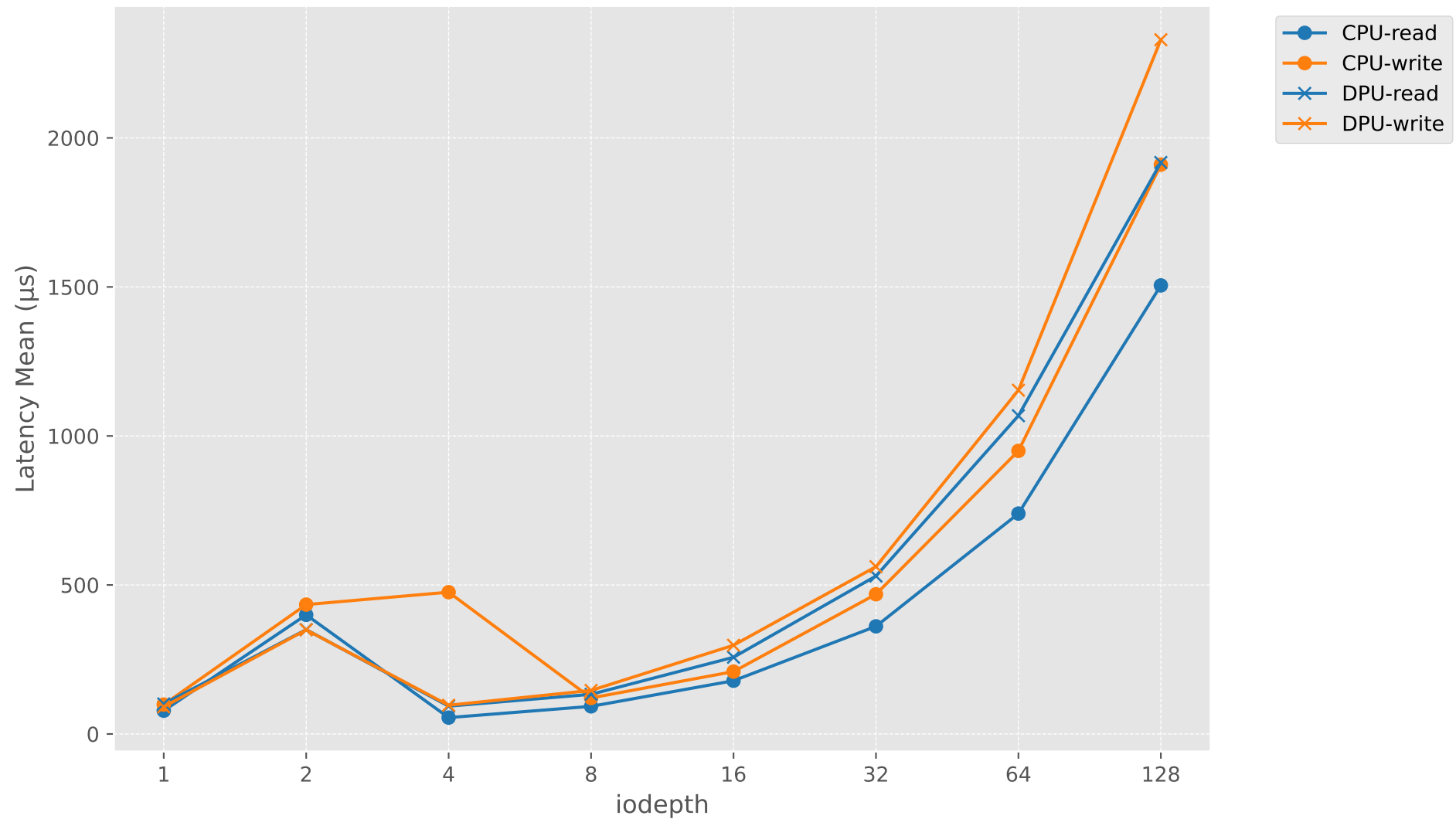
Latency Mean vs iodepth (Sequential)
